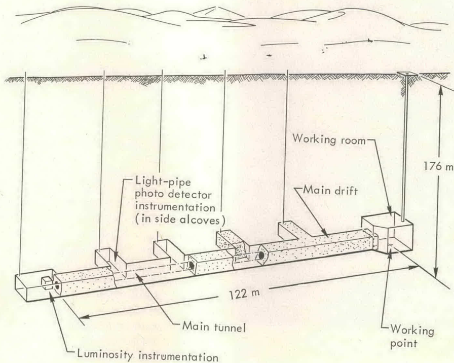
Fig. 1. General design of the Marvel experiment.
