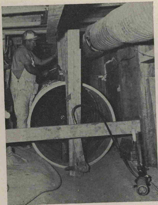
Fig. 2. Installation of the Transite pipe in the main drift. The concrete trough was first poured and cast to facilitate proper alignment of the Transite pipe sections.
